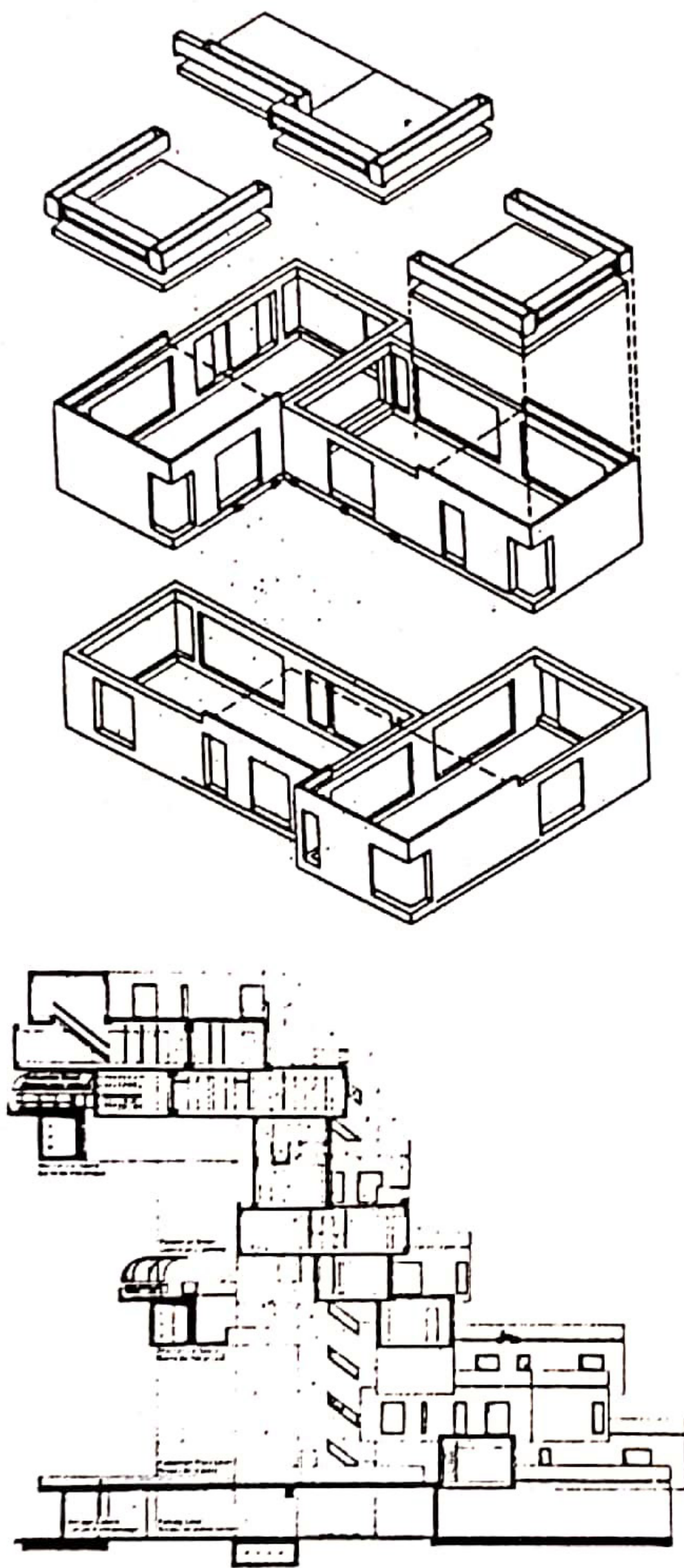
Moshe safdie Habitat 67, first phase, Montreal 1964-67.
