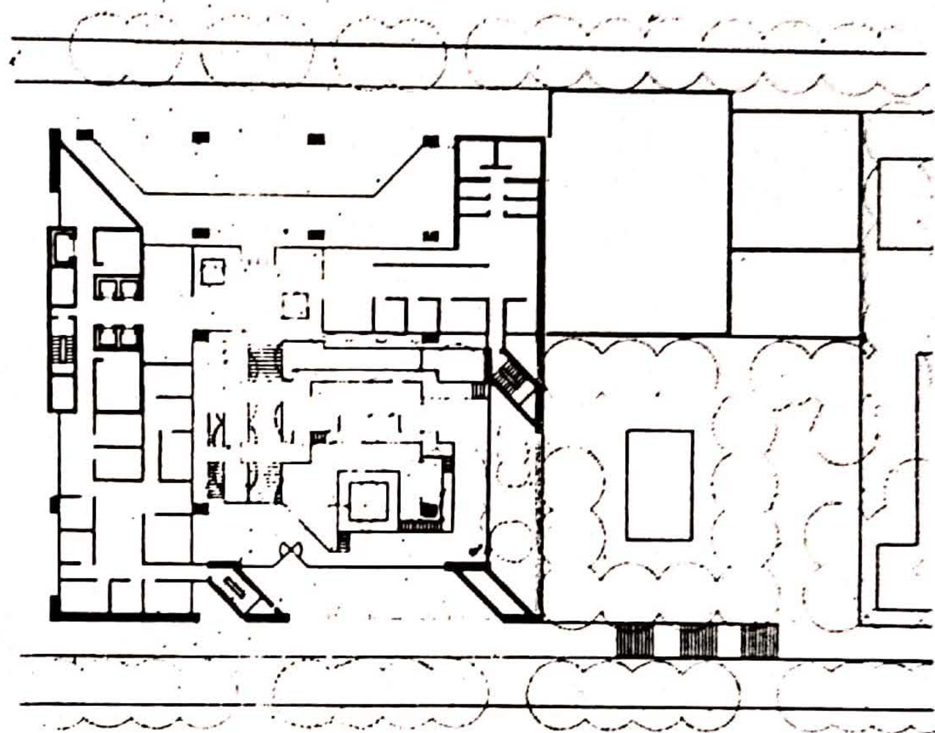
Plann tenth floor
