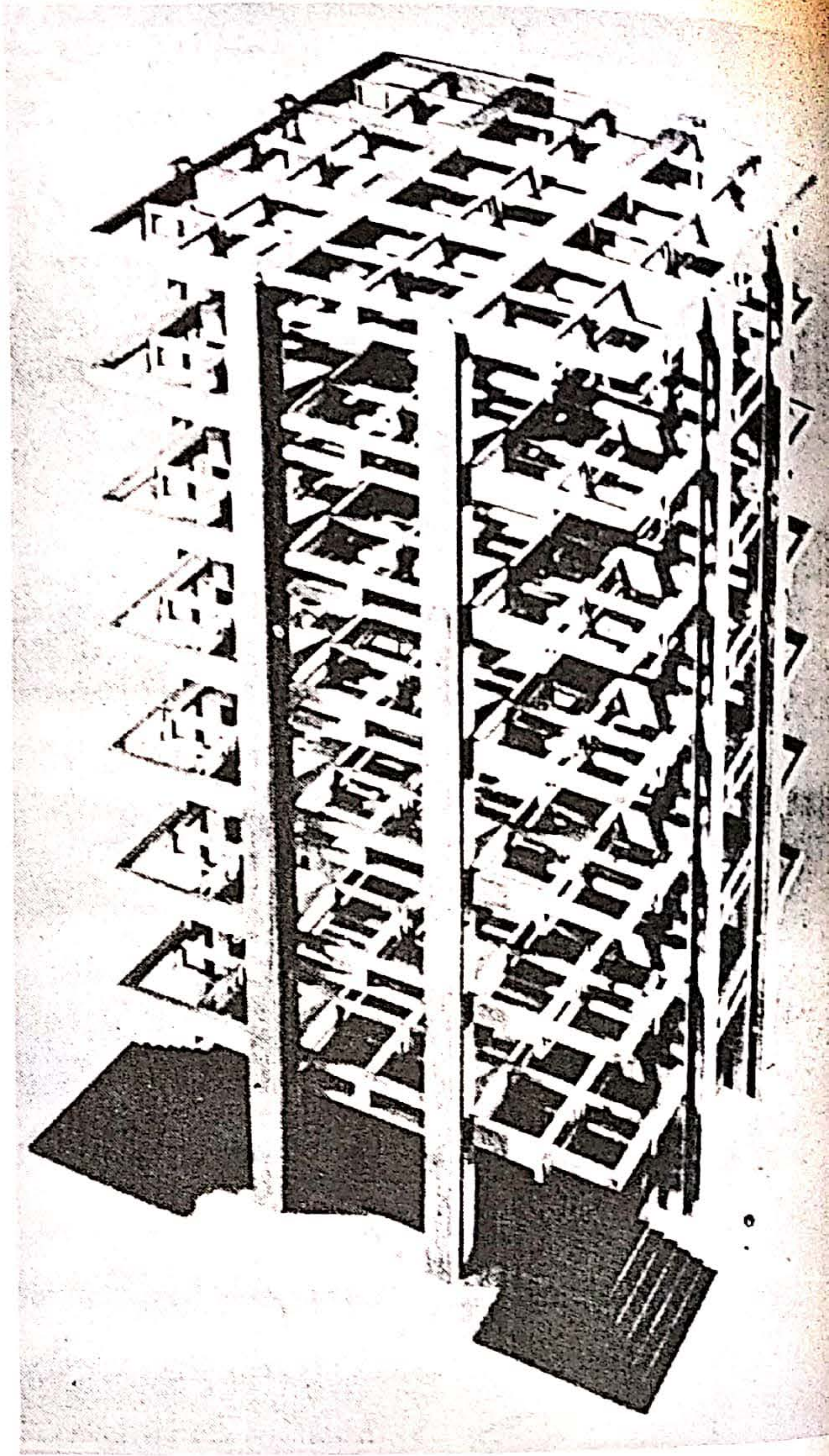
Kahn-Richards Laboratories University of Penn. Structural Concept.
